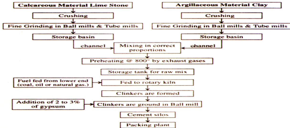
FLOW CHART FOR DRY-PROCESS OF CEMENT MANUFACTURING
