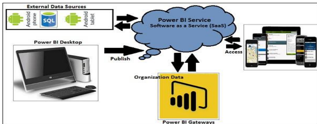
Fig 1 : The Components of Power BI
